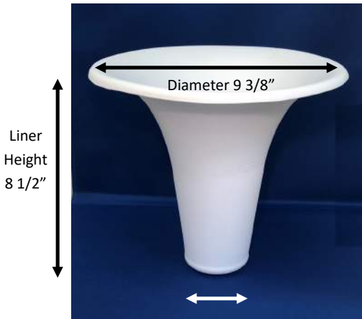
Bottom Diameter 2 3/4"
